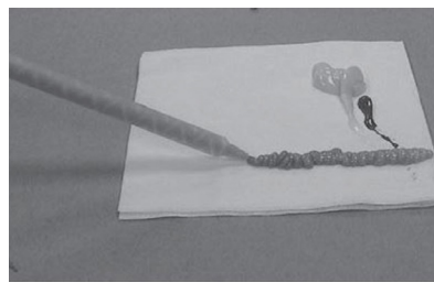
Dispense mixer length of adhesive on scrap material to ensure proper mix
