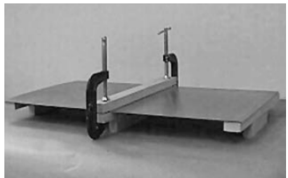
Figure 12 – Braces
