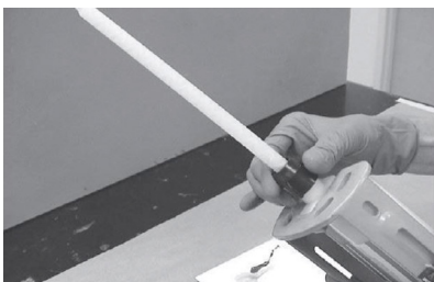
Attach static mix tip to cartridge
